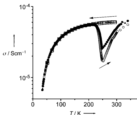
Figure 5. Electrical conductivity of gold nanoparticle assemblies linked by 3 as a function of temperature cycling. The first data collection was cycled between 294 and 4.2 K, and the second data collection was cycled between 340 and 4.2 K. The arrows indicate the direction of the temperature change. □ = first cooling; ○ = first warming; ▲ = second cooling; ● = second warming.
